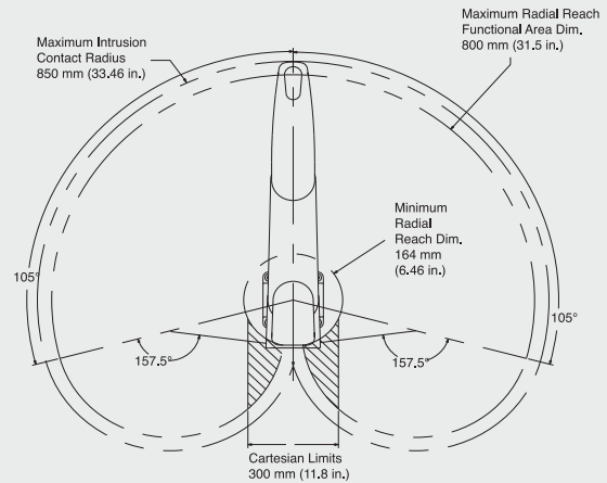
Work Envelope
